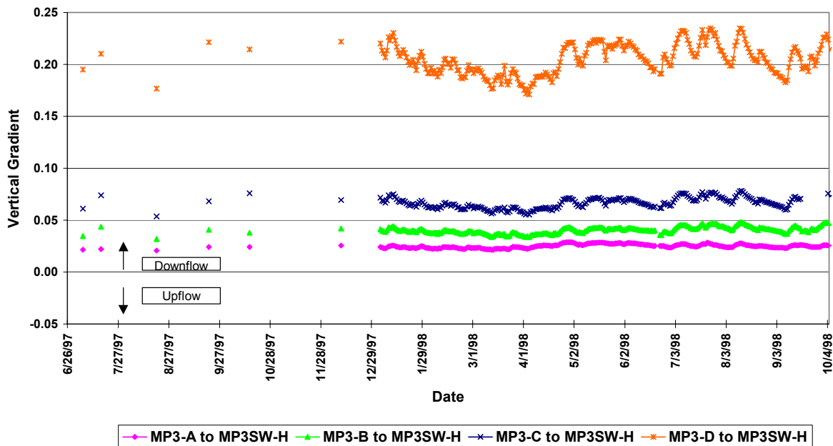
Figure 73. ENR site MP3. Water levels and vertical hydraulic gradients. Vertical gradients are calculated relative to each well and to surface water. A positive gradient indicates the potential for downward flow.
