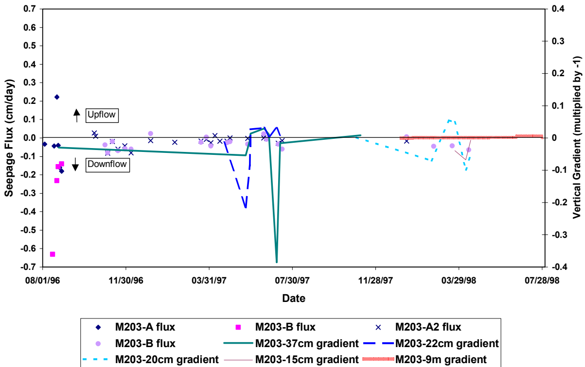
Figure 141. ENR sites M207 and M203. Seepage meter flux measurements and vertical hydraulic gradients. A positive flux indicates upward flow across wetland sediment surface. A positive gradient (after multiplying by -1) also indicates upward flow.
