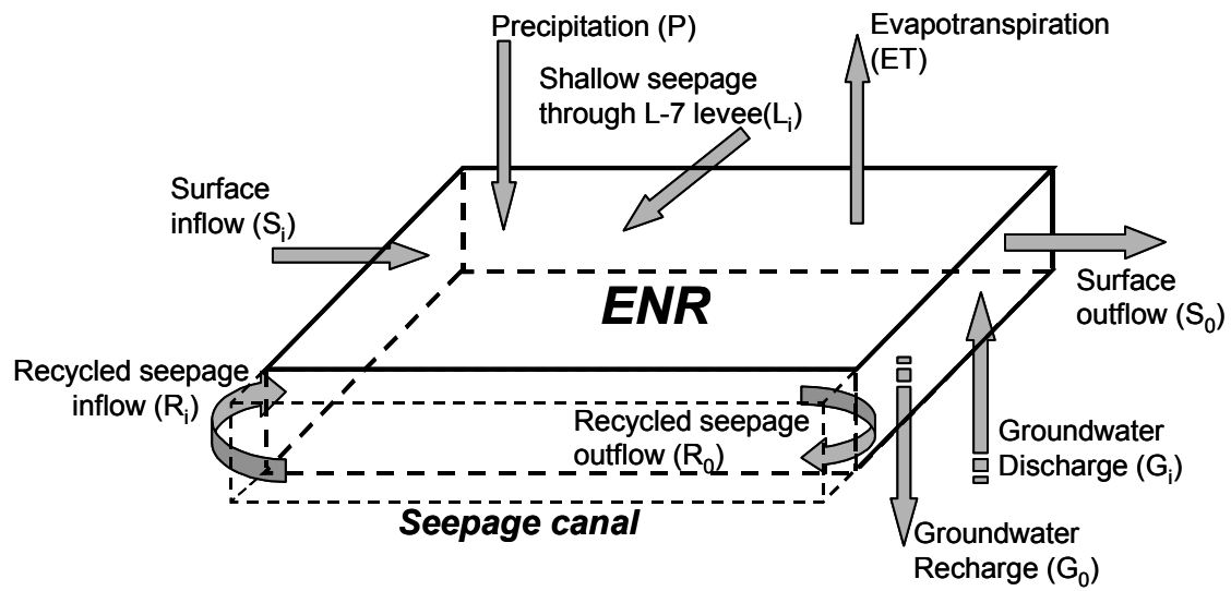
Figure 152. Conceptual model of water flows in the ENR Conceptual model of water flows in the ENR.
